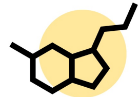
Serotonin
