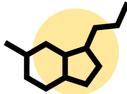
Serotonin
